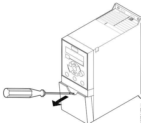
Figure 1.3 Removing Terminal Cover
