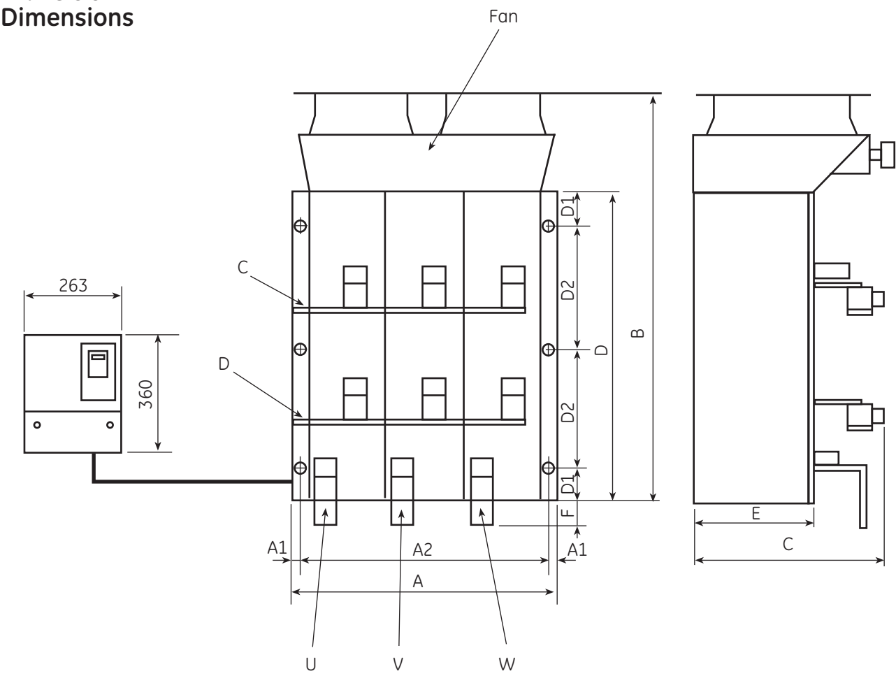
Mechanical Dimensions of 900 A...2350 and Q2 Sizes
