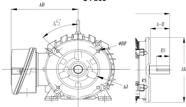
C-Face
